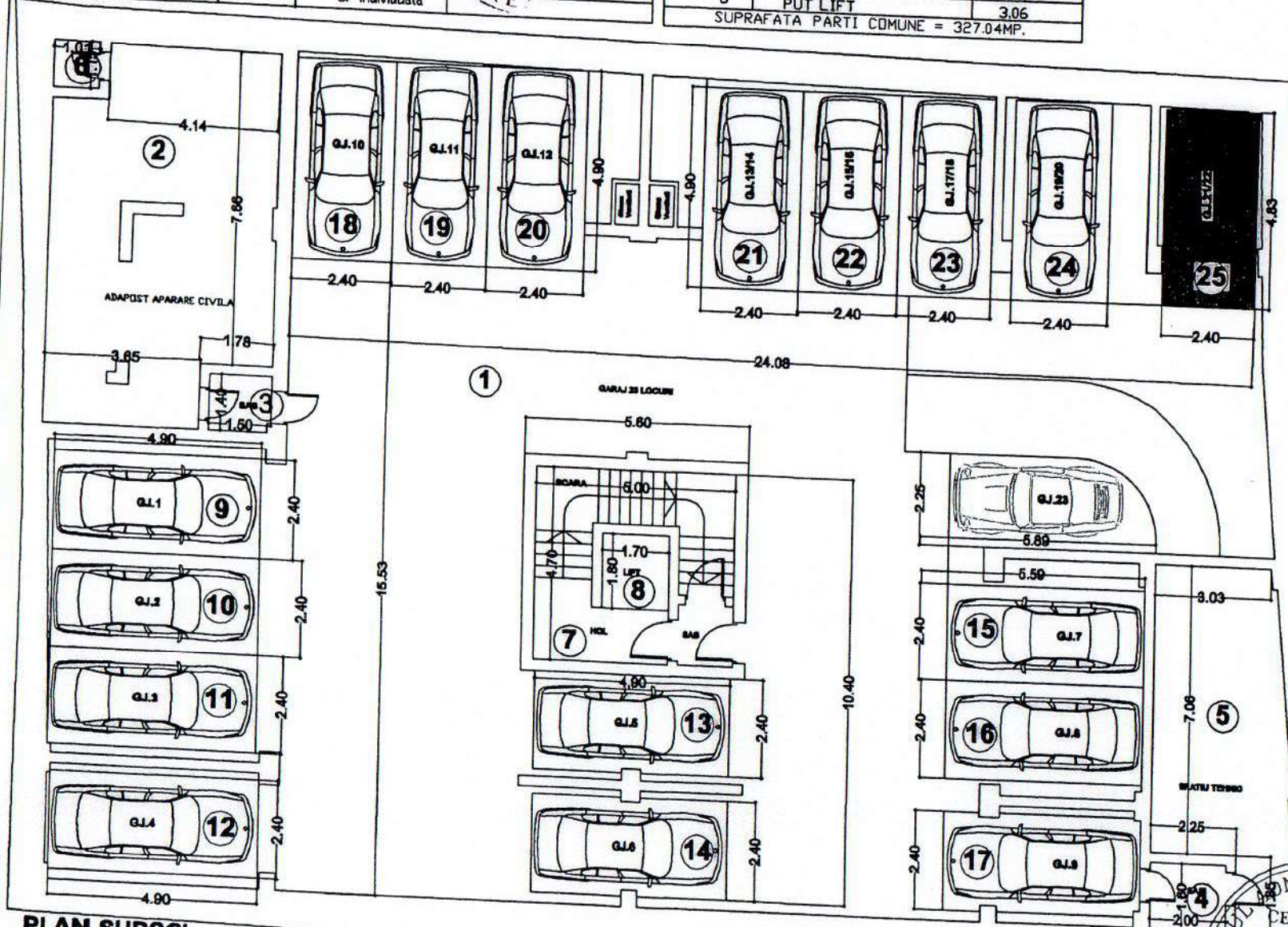
PLAN SUBSOL
