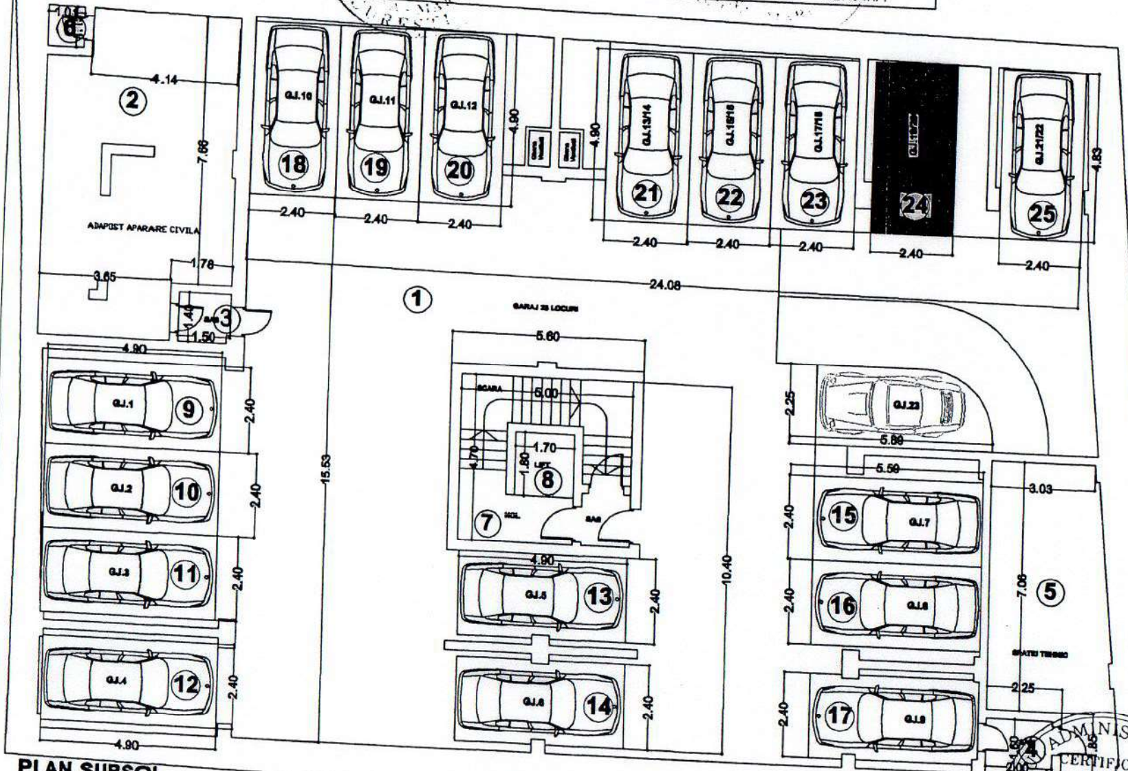
PLAN SUBSOL
