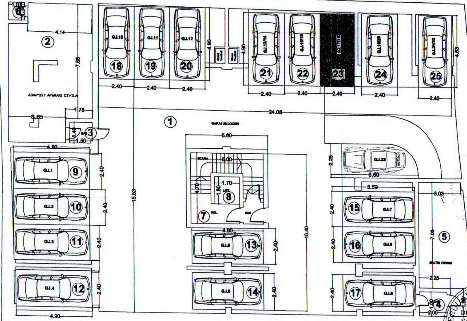
PLAN SUBSOL
